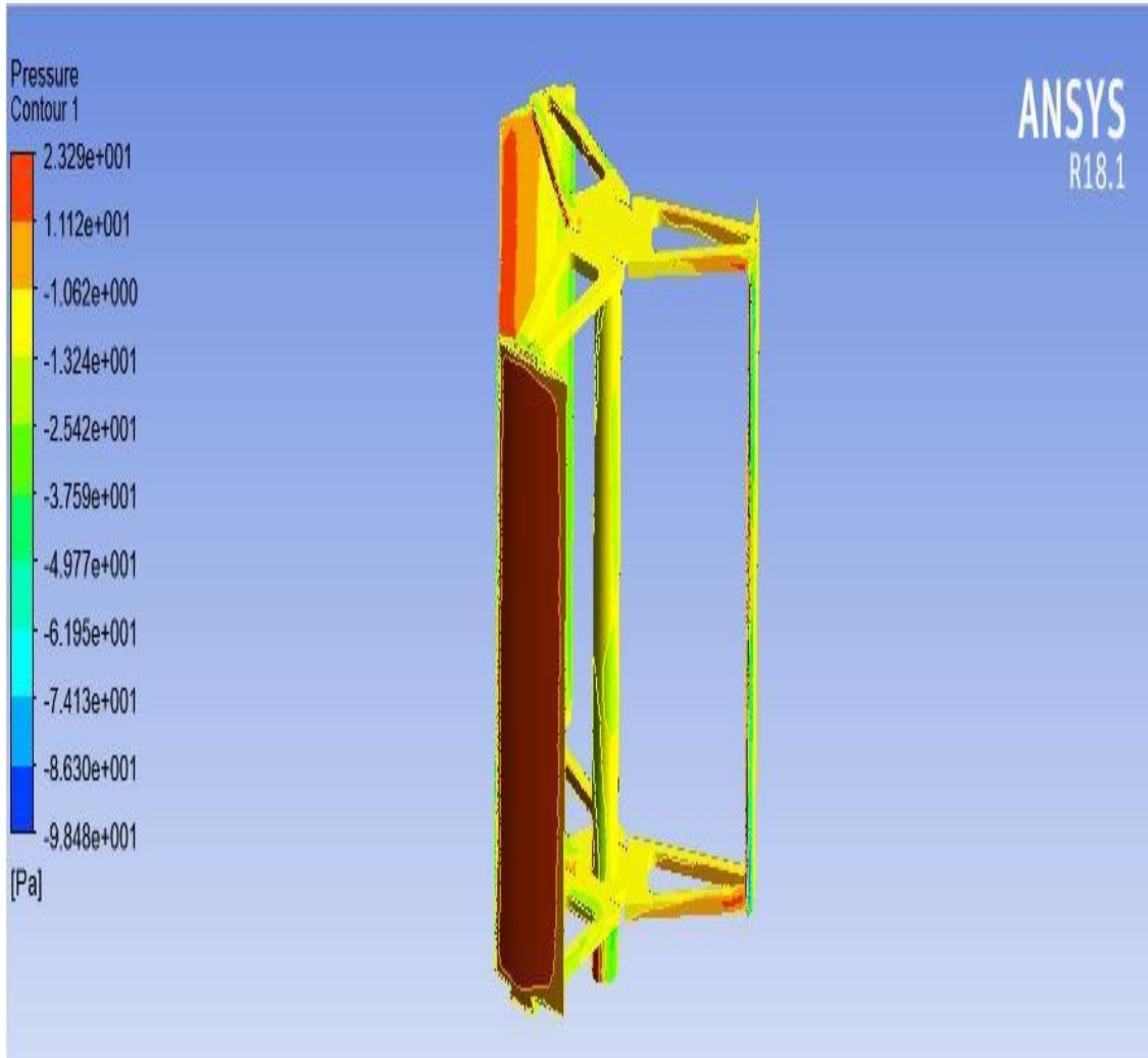
Figure 13:- Pressure Contours
