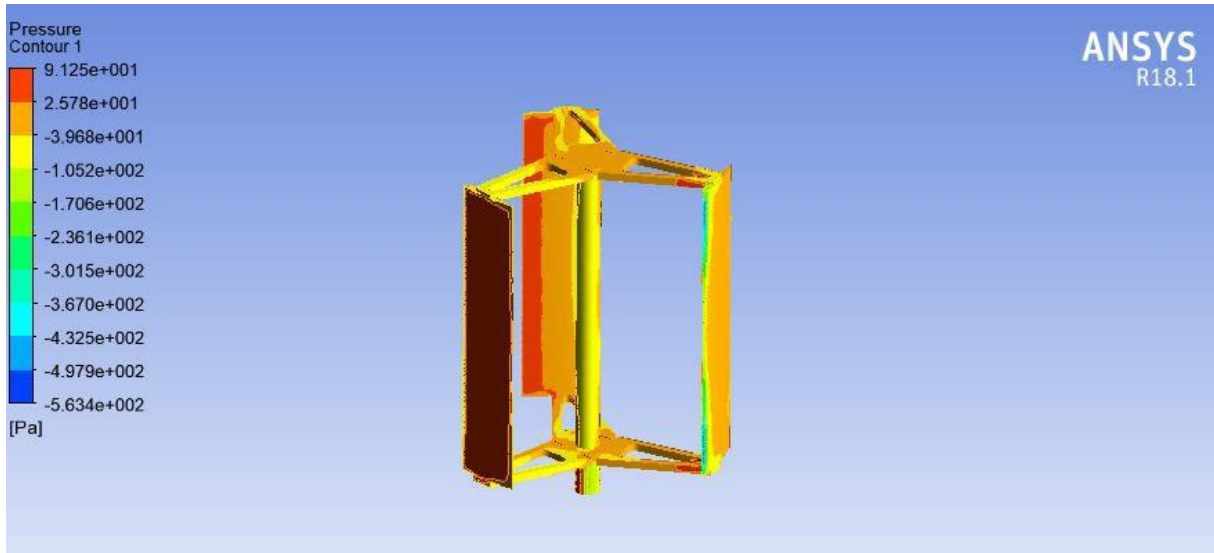
Figure 11:- Pressure Contours
