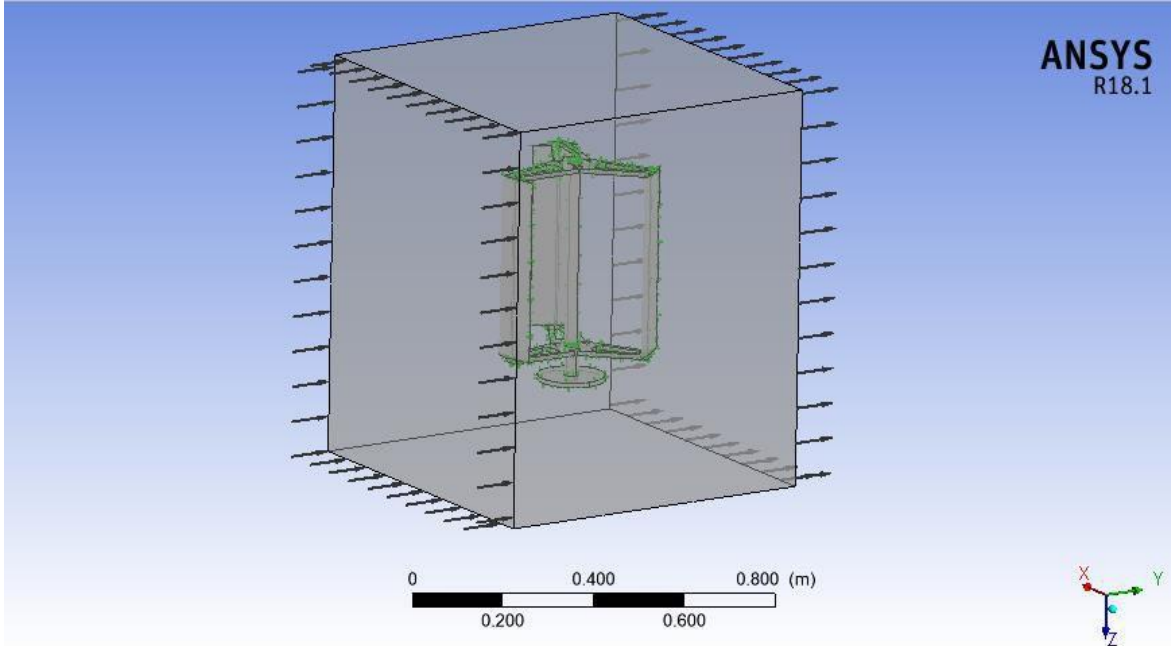
Figure 9:- Loads And Boundary Condition
